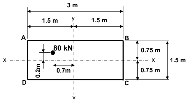
Fig. 20.9 Example of eccentric foundation loading.
