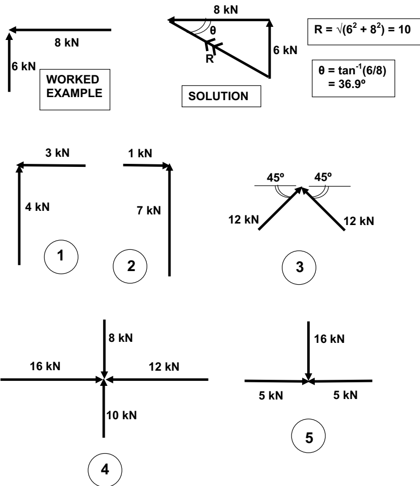
Fig. 7.6 Components: examples.
