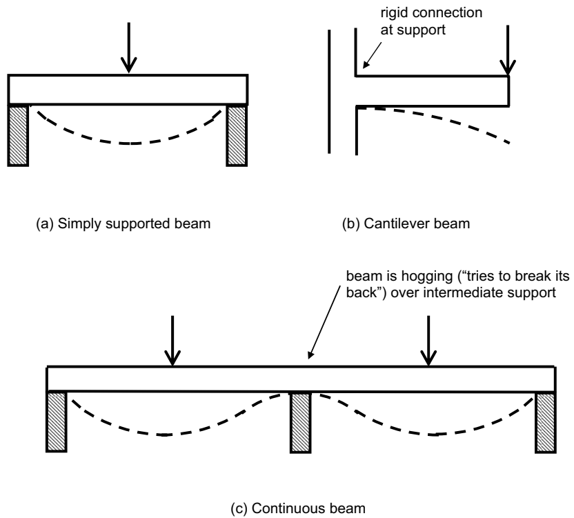
Fig. 3.6 Beam types.
