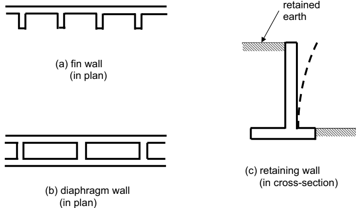
Fig. 3.9 Wall types.
